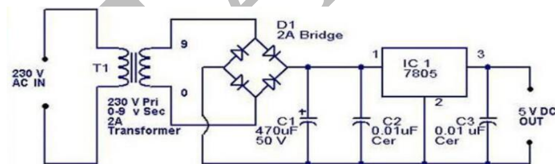
Fig. 8: 5volt Power Supply
