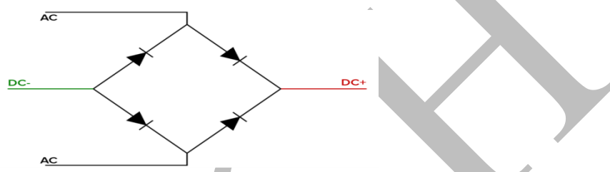
Fig. 5: bridge rectifier Symbols
