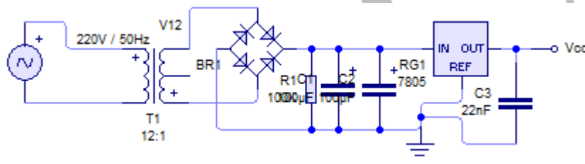
Fig .3, Power supply design with 5Volt output
