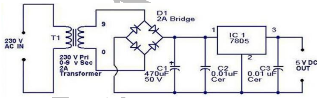
Fig. 8: 5volt Power Supply
